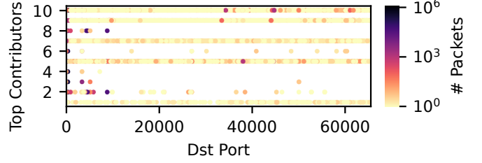
Fig. 9. TCP destination ports of internal erroneous traffic generated by the top-10 contributors.
