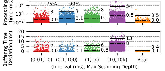
Fig. 12. Periodic check of timeout expiration for various configurations of ( P_{DT} , d_{max} ), with DT timeout set to 1s. “Real” refers to the deployment in our campus network.
